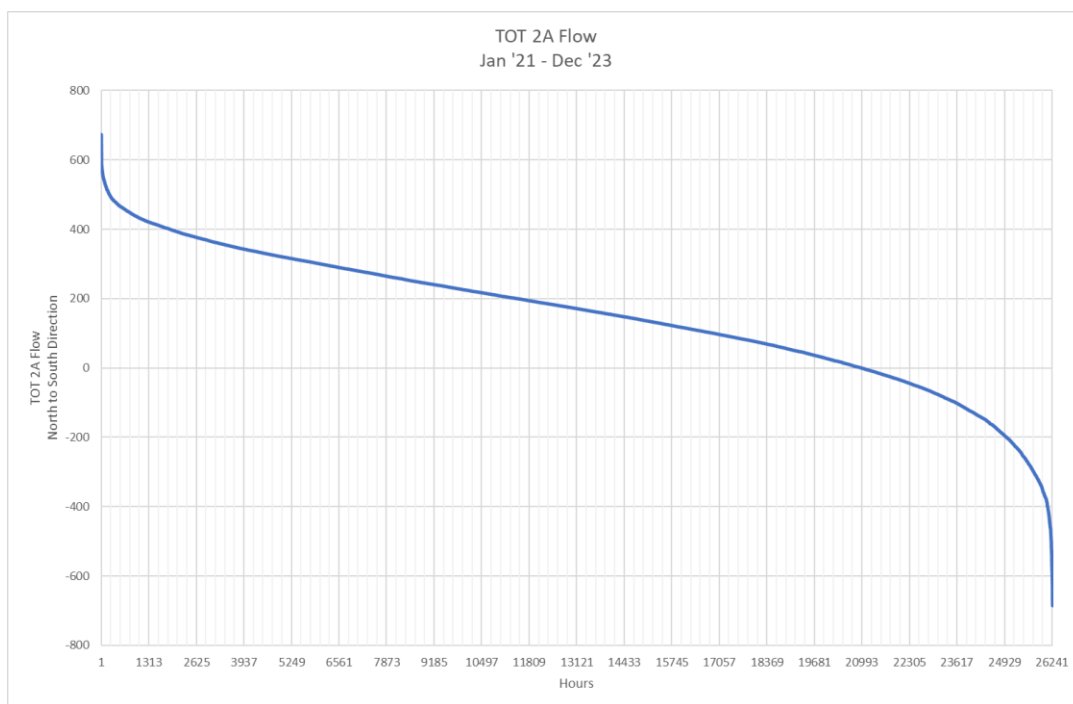
Figure 2: Hourly Distribution of TOT 2A Flows, January 2021 thru December 2023
